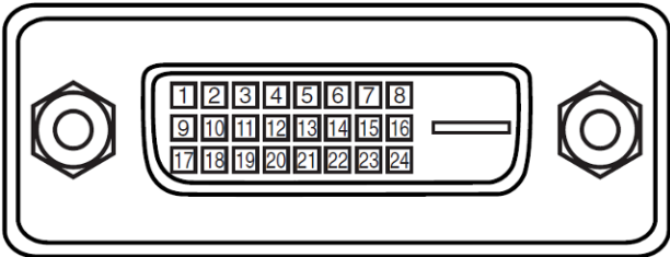
DVI-D Terminal
