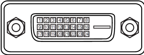
DVI-D Terminal
